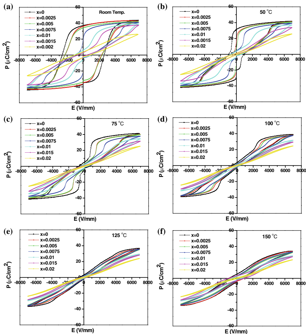
Fig. 6 P - E hysteresis loops of BNTBT6 + x Nb ceramics measured at various temperatures
