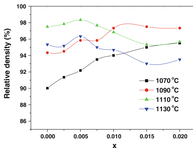
Fig. 2 Sintering behavior of BNTBT6 + x\text{Nb} samples as a function of \text{Nb}^{5+} content and sintering temperature as indicated
