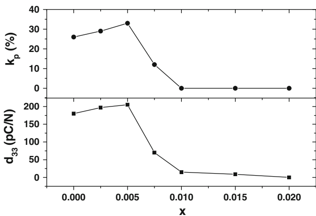
Fig. 7 Piezoelectric properties of BNTBT6 + x Nb ceramics as a function of Nb^{5+} content x
